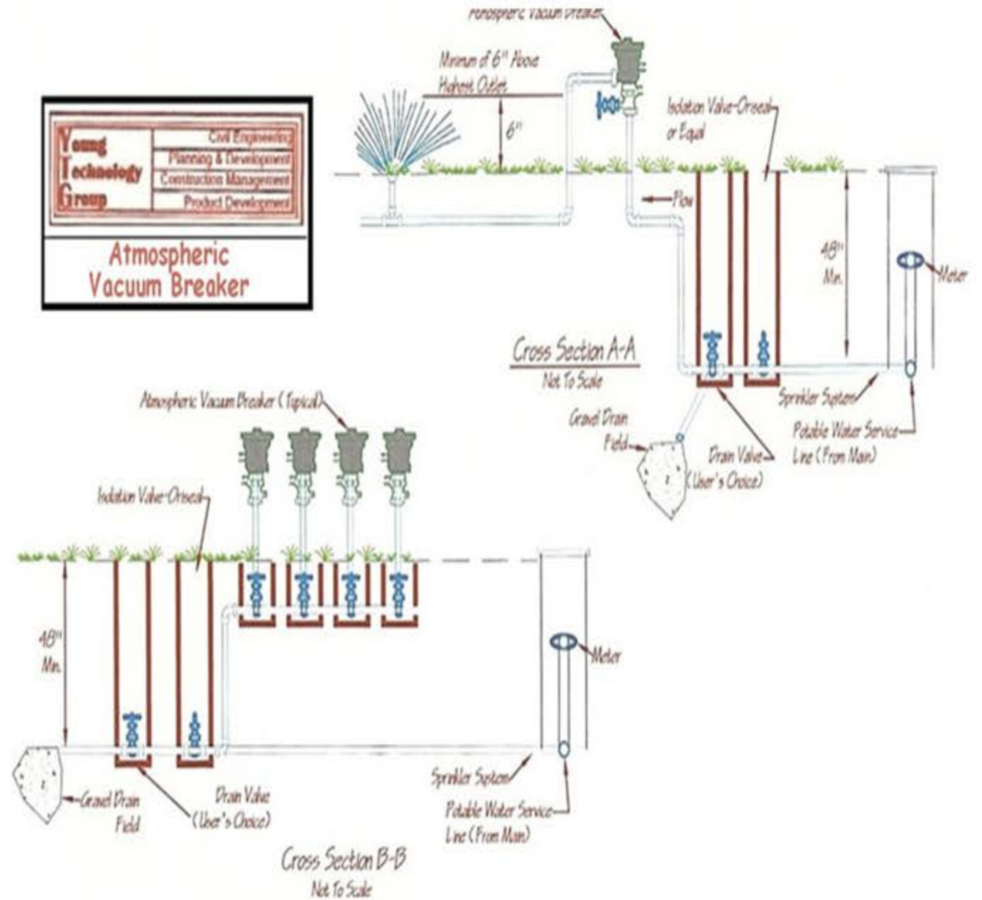
Section View: Atmospheric Vacuum Breaker
