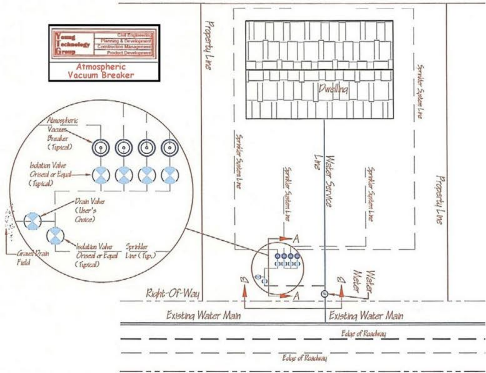
Plain View: Atmospheric Vacuum Breaker
